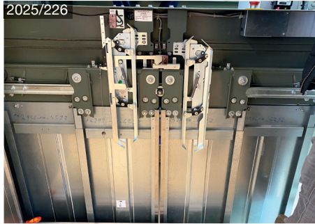
Schindler Varidor35 center
