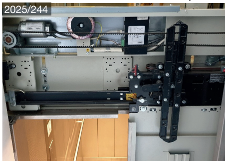
Sematic 2000 Code B105AANX telescope
