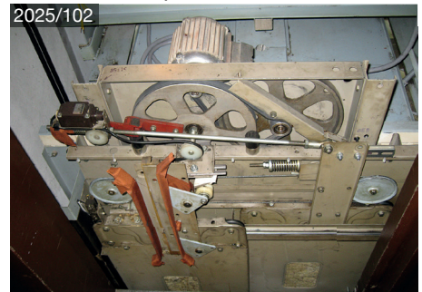
Kone ADR telescope
