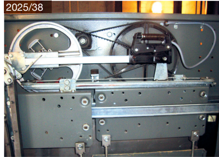
Fermator Sinus telescope
