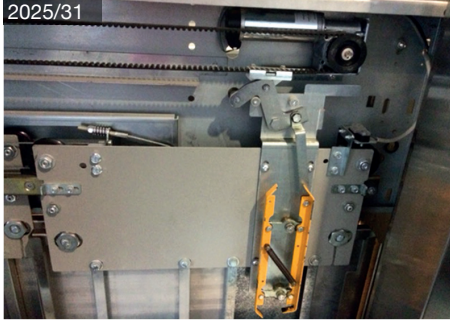
ELEX Aurex
