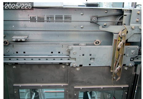
Schindler Varidor 50 telescope
