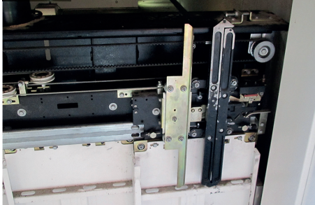
Liftcomp telescope
